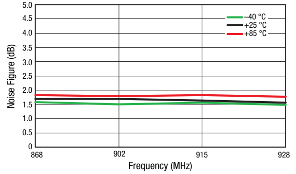
Figure 16. Receive Path Noise Figure (LNA_IN to RFIO) vs Frequency Over Temperature
